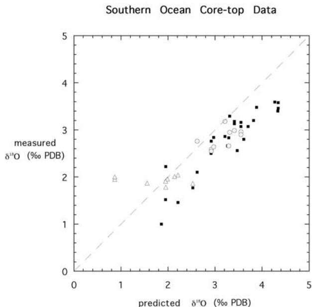
Figure 7. Plot of measured \delta^{18}\text{O} (‰PDB) versus predicted \delta^{18}\text{O} (‰PDB) for Southern Ocean core-top data compiled from both Labeyrie et al. [1996] and this study. Predicted values are all derived from austral summer temperature and salinity data in order to minimize seasonality effects (see Labeyrie et al. [1996] and text of this study for details). Foraminiferal species shown from both the south Indian and South Atlantic sectors are G. bulloides and N. pachyderma (left-coiling). The dashed line corresponds to a 1:1 slope where measured values follow those that are predicted. N. pachyderma data are represented by solid squares; G. bulloides (where predicted values are > 2.6\text{‰} ) data are represented by open circles; and G. bulloides (predicted values < 2.6\text{‰} ) data are represented by open triangles. Note that the N. pachyderma and the G. bulloides (predicted > 2.6\text{‰} ) data follow the 1:1 slope, while the G. bulloides (predicted < 2.6\text{‰} ) data do not, indicating that G. bulloides \delta^{18}\text{O} from warmer regions farther north are typically heavier than predicted, a pattern that does not occur farther south (see text for details). One of the G. bulloides data points (predicted value of 0.87\text{‰} ) comes from a core location close to TNO57-21 and is not presented elsewhere in this study.
