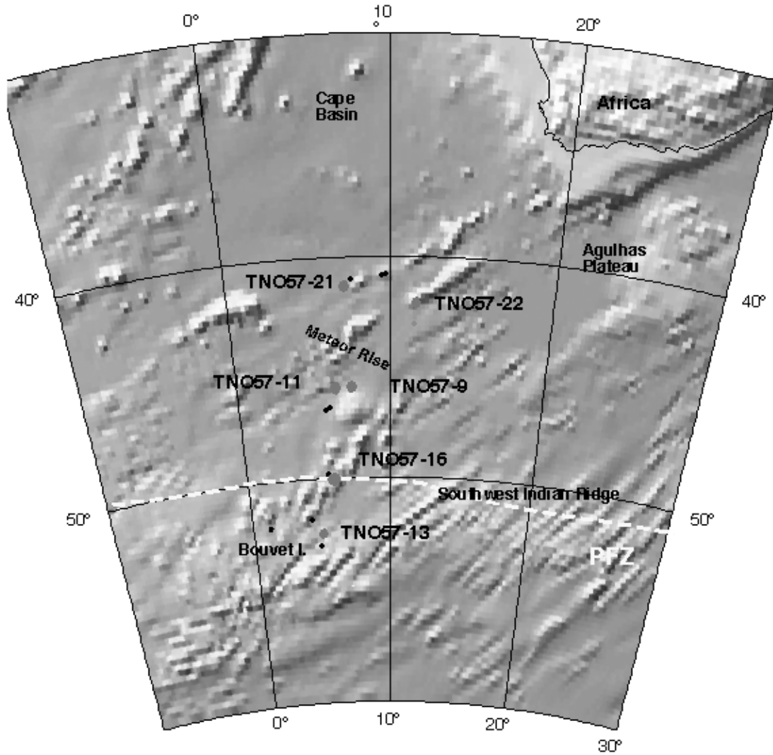
Figure 1. Map showing our plankton tow station locations between Africa and Antarctica. The dashed line corresponds to the mean position of the modern Polar Frontal Zone (PFZ), which is the northern terminus of the subsurface T_{\min} layer bounded by the 2^{\circ}\text{C} isotherm in the 100–300-m layer in the summer and the vertical 2^{\circ}\text{C} isotherm in the winter [Belkin and Gordon, 1996].
